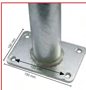
Bottom Plate
